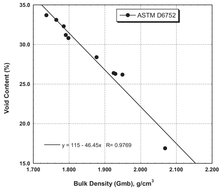
Figure 5. Plot of Void Content and Bulk Density of Pervious Concrete as Determined Using Vacuum Sealing Method ASTM D6752
