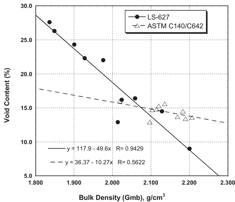
Figure 4. Comparison of MTO LS-627 and ASTM C140/C642 Test Results for Bulk Density and Void Content for Pervious Concrete
