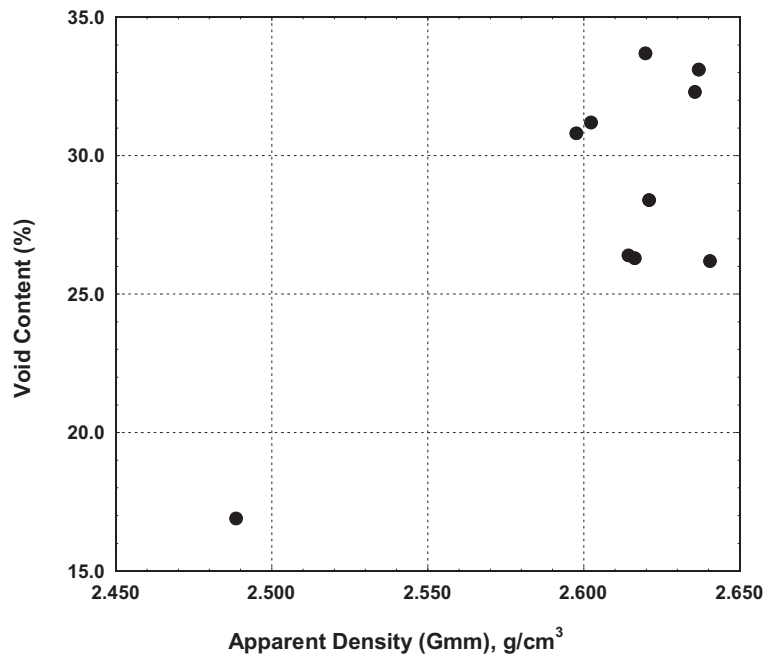
Figure 6. Plot of Void Content and Apparent Density of Pervious Concrete as Determined Using Vacuum Sealing Method ASTM D6857
