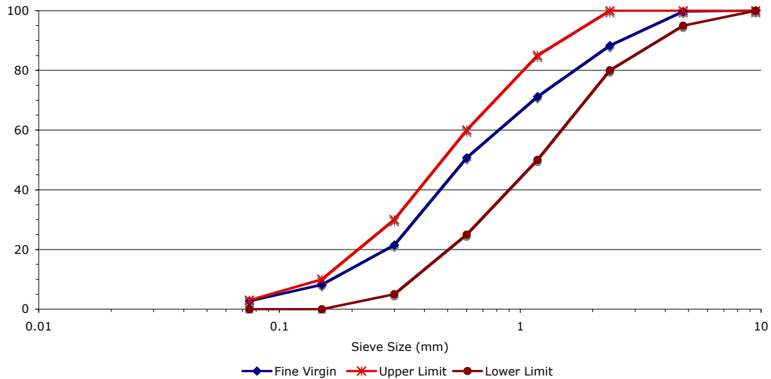
Figure 4. Fine Aggregate Grading
