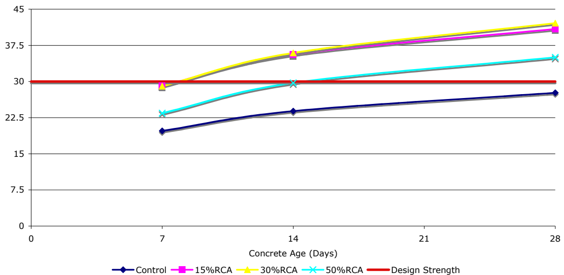
Figure 5. Compressive Strength Development
