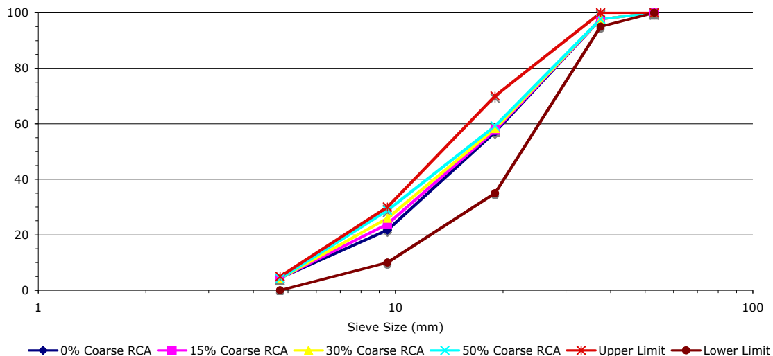
Figure 3. Coarse Aggregate Gradings
