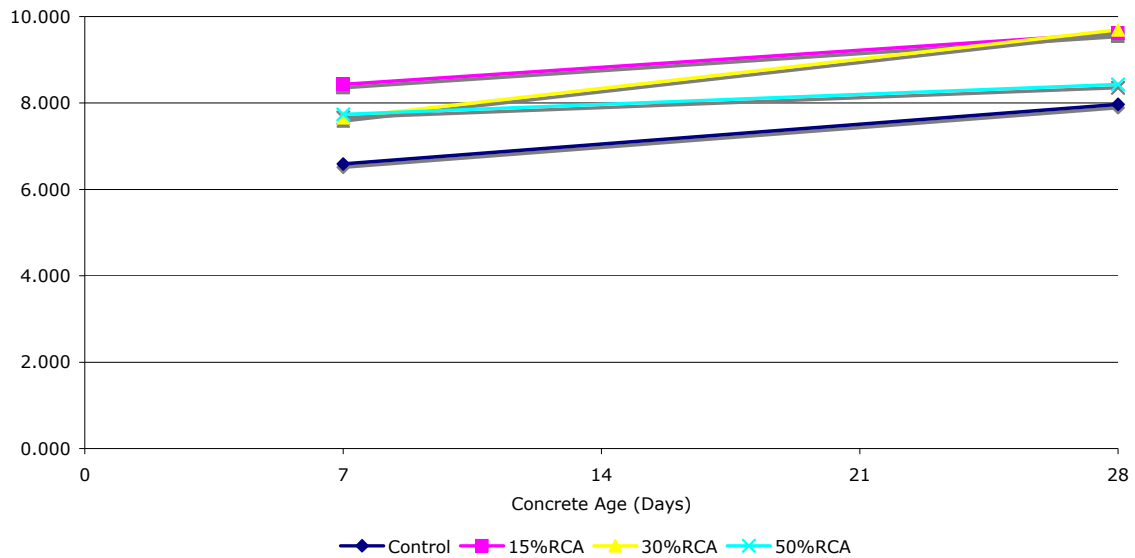
Figure 6. Flexural Strength Development
