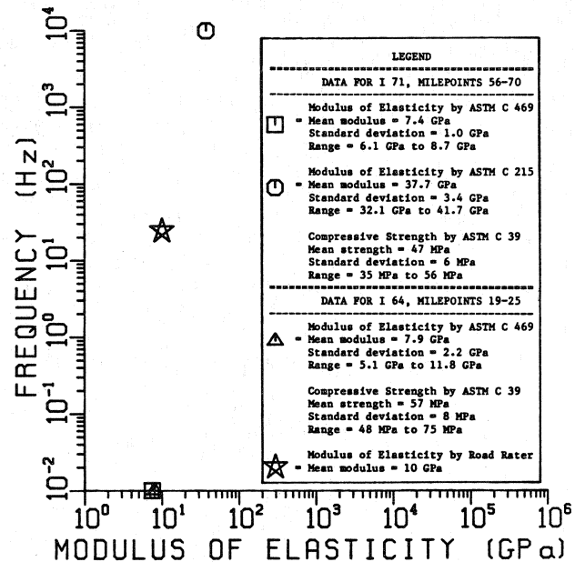
Figure 9. Modulus of elasticity versus frequency of loading.
