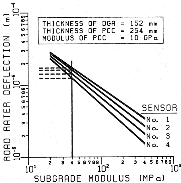
Figure 7. Deflection versus subgrade modulus.
