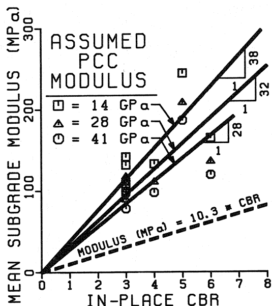
Figure 4. Average back-calculated subgrade moduli versus in-place CBR values.
