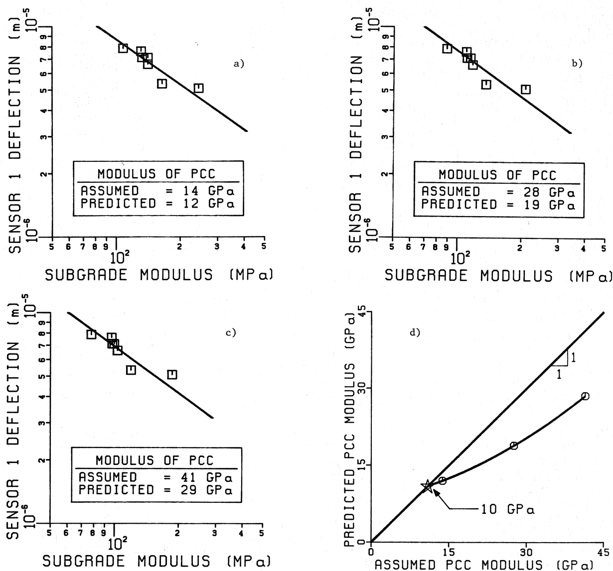
Figure 6. Estimation of effective modulus of portland cement concrete pavement.
