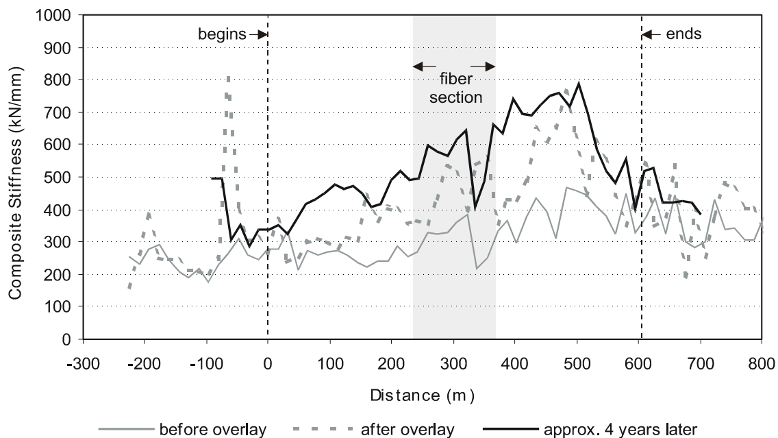
Figure 5. FWD Data of Overlay on I-85 Outside Lane
