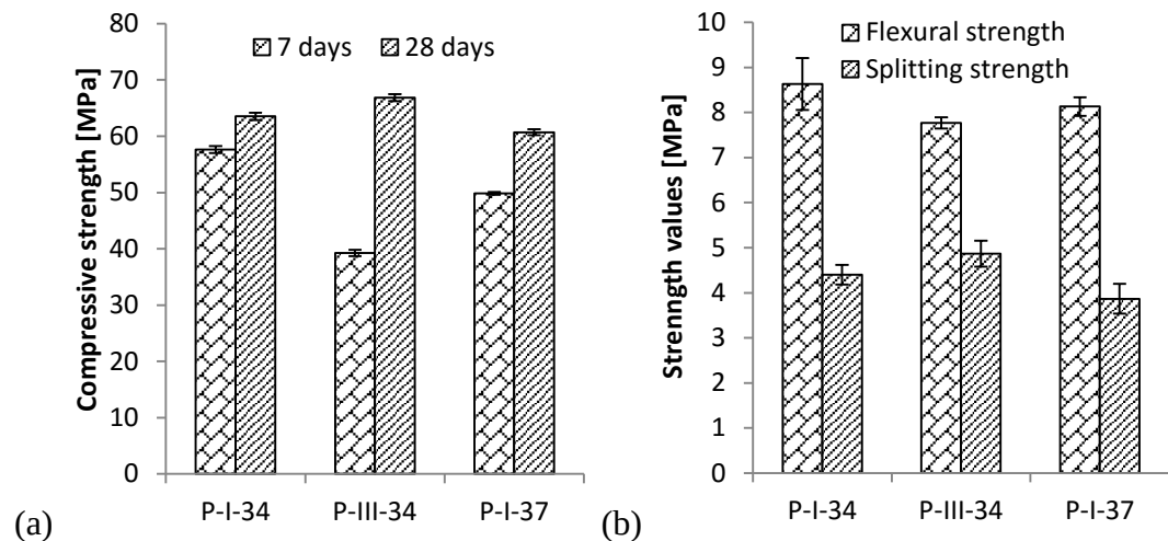
Fig. 2. Concrete strength data: (a) the compressive strength after 7 and 28 days of water curing; (b) flexural and splitting strength after 28 days of water curing.
